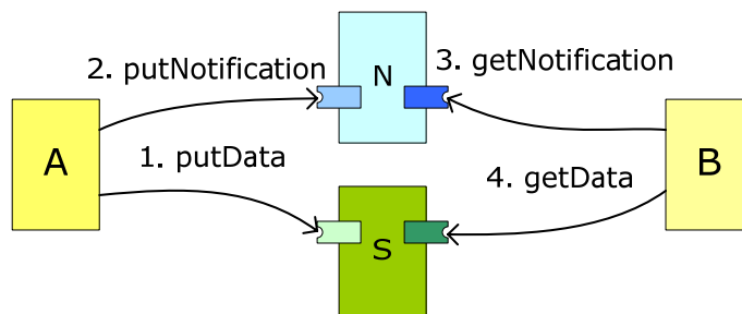
Figure 11 Deliver and notify interaction pattern
