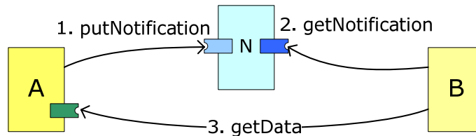
Figure 10 Notify and retrieve interaction pattern
